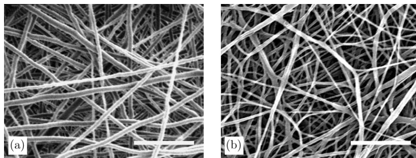
Fig. 7. Ultrastructural morphology of PCL NFS examined by SEM. (a) A PCL NFS produced by the electrospinning process showing random orientation of ultra-fine fibers with a diameter ranging from 500 nm to 900 nm, defining a matrix with inter-connecting pores. (b) A NFS incubated in culture medium at 37°C for 21 days. Both fibers and pores are maintained and no significant structural degradation is evident. Bar 10 μm. [Copyright: Ref. 74]
